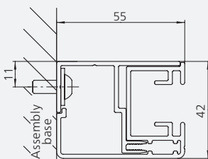
Installation in reveals
