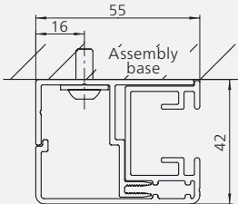
Wall mounting
